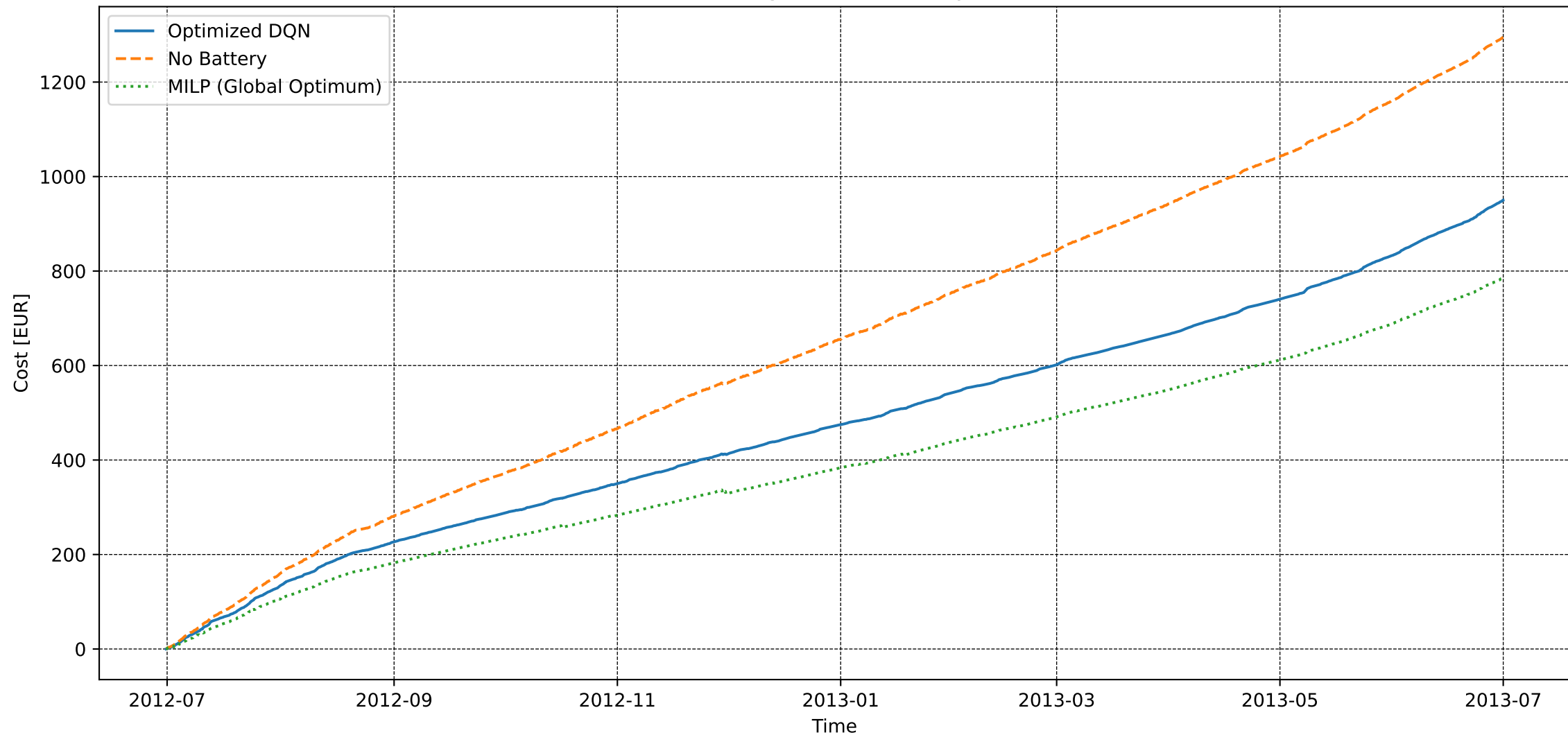
User 1 - Extended Convergence - Electricity Cost [DQN vs MILP]
